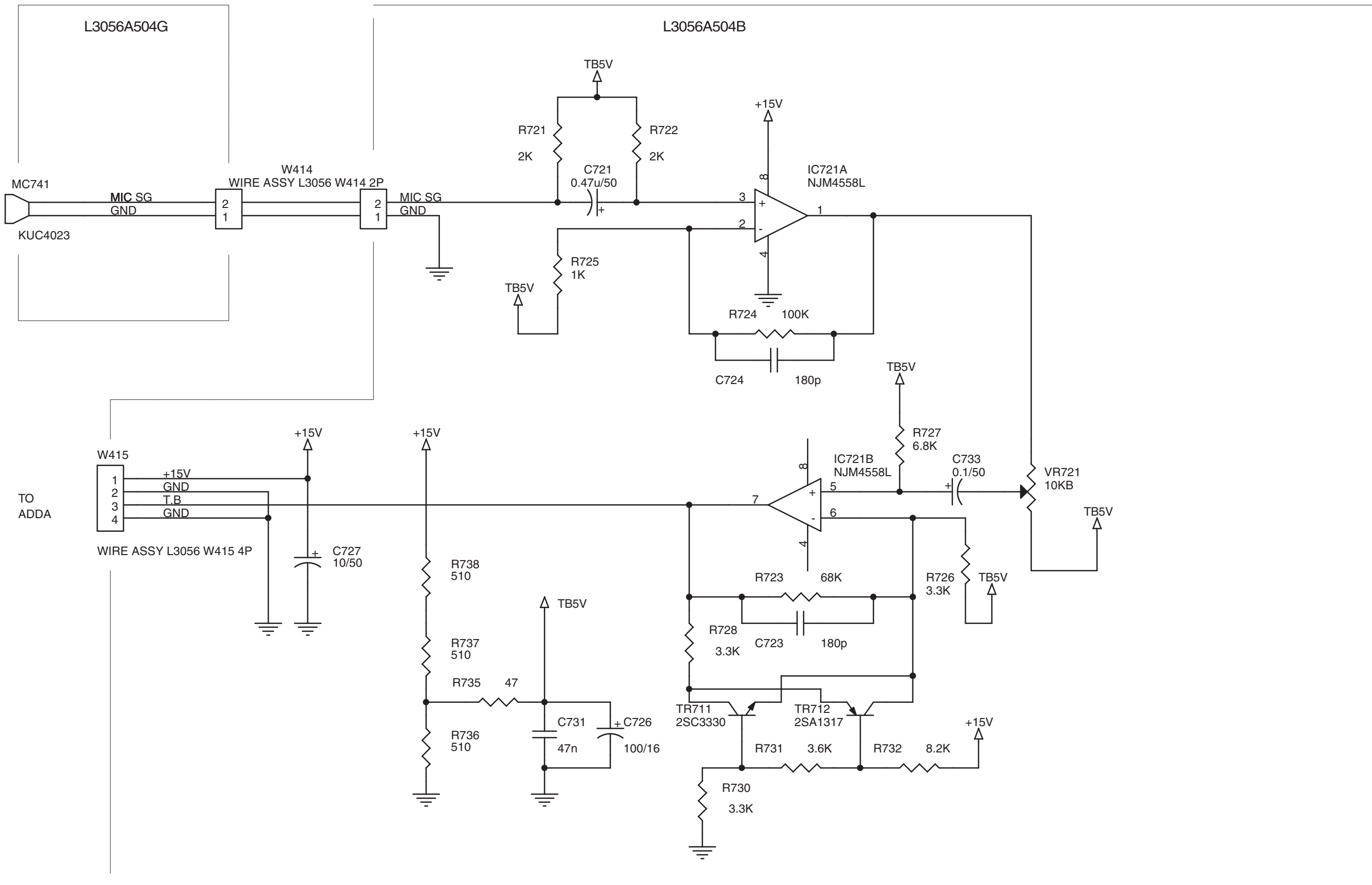
DPS24 PC 7 SEG (1/2), MIC SCHEMATIC DIAGRAM
