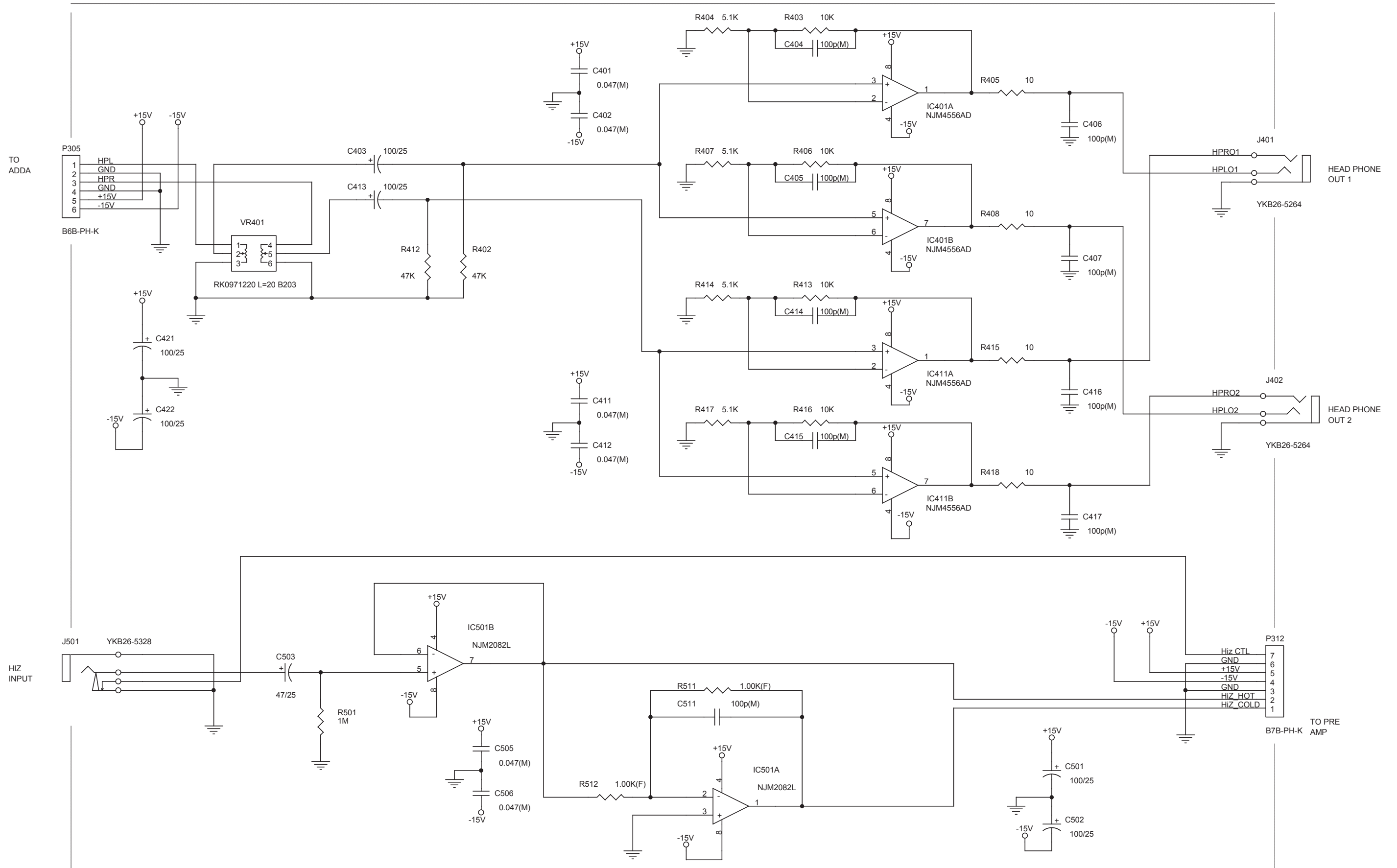
DPS24 PC HP-HIZ SCHEMATIC DIAGRAM
