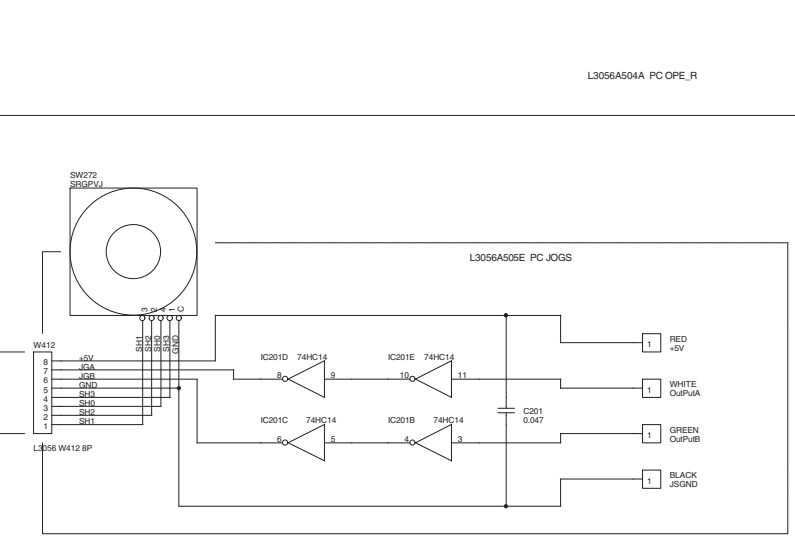
DPS24 PC OPERATION R, JOG SCHEMATIC DIAGRAM
